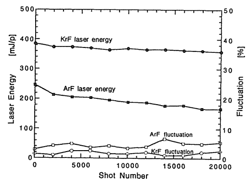
Fig. 10 Gas life of KrF and ArF laser.
