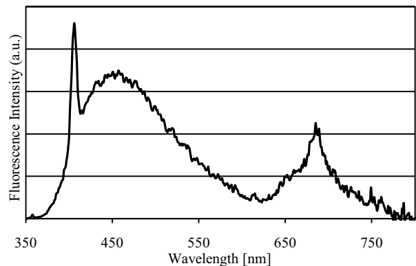
Fig. 1 Laser-induced fluorescence spectrum of water of Lake Suwa on September 18, 2009.
