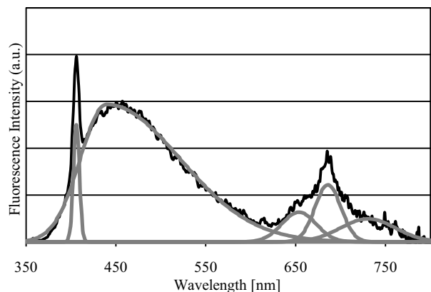
Fig. 2 Separation of fluorescence spectrum of water of Lake Suwa on September 18, 2009.
