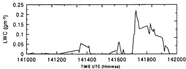
Figure 9: Liquid water content (LWC) as measured with the Johnson-Williams Liquid Water probe of the Hercules along a flight leg nearby the Falcon leg on 20 October 1998 at an altitude of 4 km.
