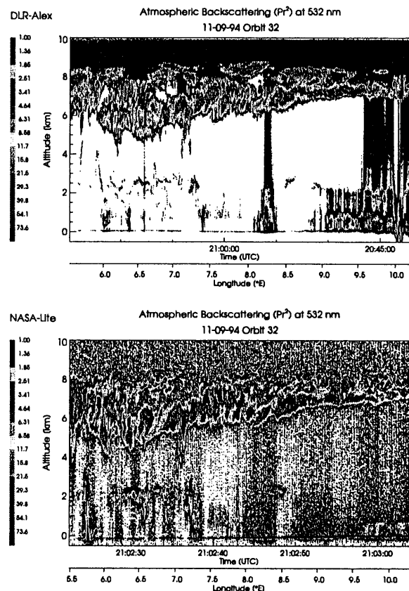
Figure 2: Backscatter cross sections at 532 nm wavelength for ALEX and LITE instrument.
