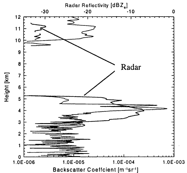
Figure 10: Radar reflectivity and lidar backscatter coefficient @ 1064nm on 20 Oct. 98, 14:32:53. The lidar data was averaged over 1 s (about 212 m), the radar data was averaged over 8 s in order to match the spatial scale.
