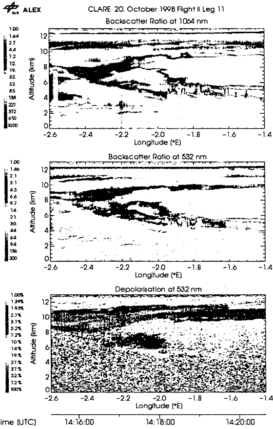
Figure 5: Lidar backscatter ratio @ 1064nm, 532nm, depolarisation ratio at 532nm on 20 Oct. 98, 14:15 - 14:21 UT. Chilbolton is located near -1.43E .
